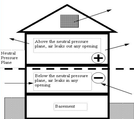
As Warm Air Rises and Leaks Through the Attic It Pulls Cold Air Into The House Below Through Windows, etc.
